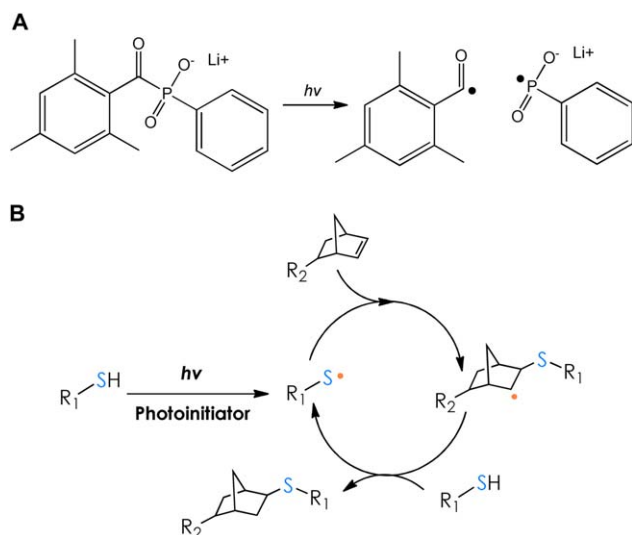
Figure 1. (A) Photocleavage of the type I photoinitiator lithium arylphosphinate into radicals. (B) Schematics of a radical-mediated step-growth thiol–norbornene photoclick reaction with a thiol-containing molecule ( R_1 -SH) and a norbornene-functionalized macromer ( R_2 -norbornene). h\nu indicates light irradiation. [Color figure can be viewed in the online issue, which is available at wileyonlinelibrary.com .]
