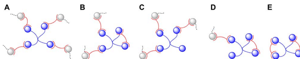
Figure 2. Schematics of the potential products after step-growth thiol–norbornene reactions between tetrafunctional PEGNB and bifunctional DTT: (A) defect-free, fully crosslinked thiol–norbornene network; (B) fully reacted thiol–ene network with a primary cycle; (C) partially crosslinked thiol–ene network with an unreacted, dangling PEGNB arm; (D) dangling polymer with a primary cycle and an unreacted PEGNB arm; and (E) soluble polymer with fully reacted functional groups. D and E did not contribute to network crosslinking. [Color figure can be viewed in the online issue, which is available at wileyonlinelibrary.com .]
