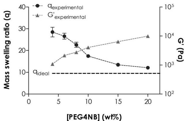
Figure 3. Effect of the PEG4NB macromer concentration on thiol–ene hydrogel equilibrium swelling (left y axis) and elastic modulus (right y axis). The swelling ratio of an ideal network was calculated on the basis of the molecular weight between crosslinks of given macromer molecular weights (molecular weight of PEG4NB = 20 kDa, molecular weight of DTT = 154 Da) and functionalities (functionality of PEG4NB = 4, functionality of DTT = 2). The ideal swelling ratio ( q_{ideal} ) was calculated on the basis of the known macromer structure and Flory–Rehner theory ( q : swelling ratio; G' : shear modulus). Reprinted with permission from 36. Copyright 2012 American Chemical Society.
